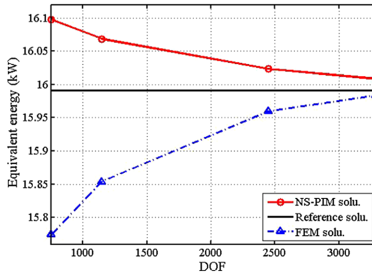
Fig. 12. Upper and lower bound solutions of the 3D engine pedestal obtained using the present NS-PIM and linear FEM, respectively.
