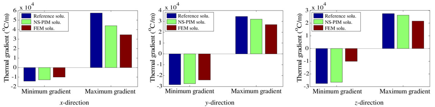
Fig. 11. Comparison of peak temperature gradient for both NS-PIM and linear FEM.
