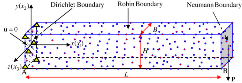
Fig. 3. Discretized model of a 3D conduction beam subjected to Dirichlet, Neumann and Robin boundary conditions on left, right and top surfaces, respectively.
