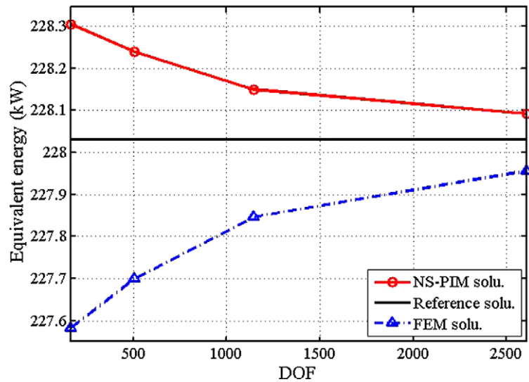
Fig. 7. Upper and lower bound solutions of the 3D conduction beam obtained using the present NS-PIM and linear FEM, respectively.
