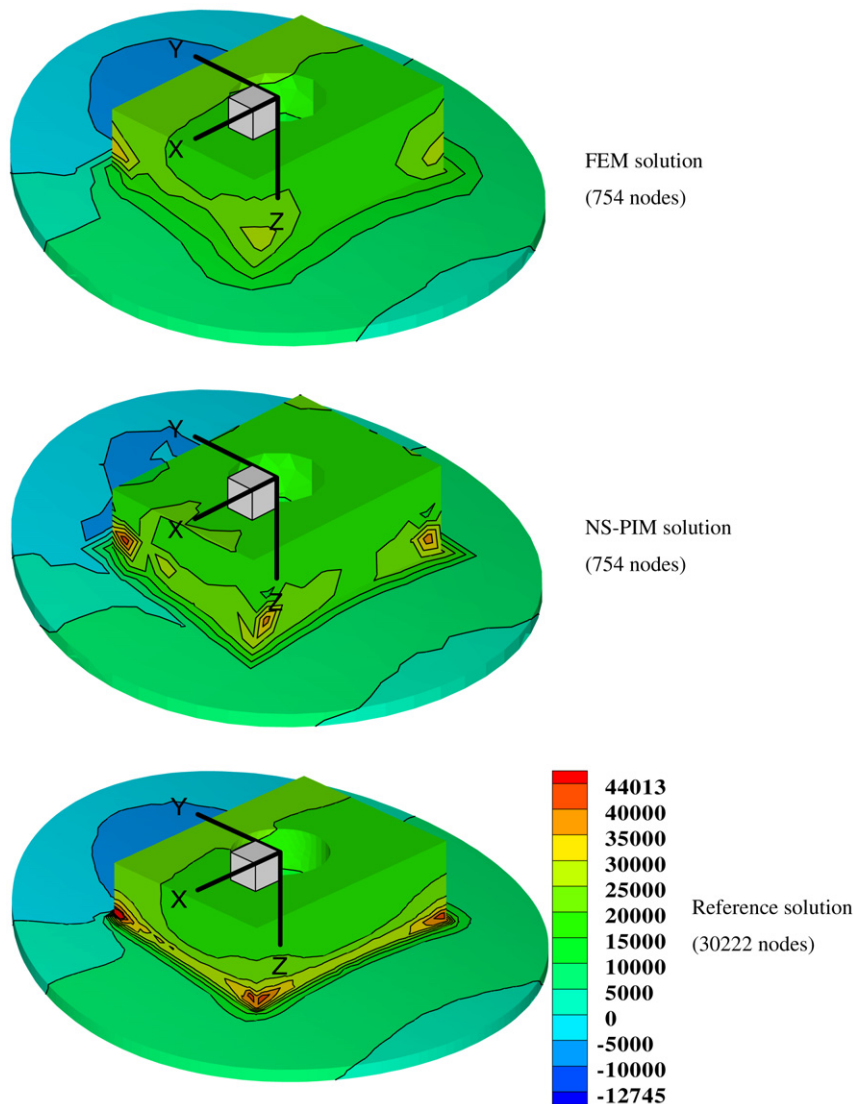
Fig. 10. Comparison of temperature gradient in z-direction.
