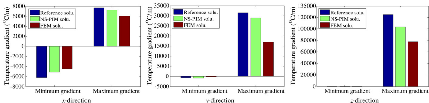
Fig. 6. Comparison of peak temperature gradients between present NS-PIM and linear FEM.
