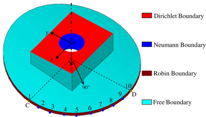
Fig. 8. Illustration of the complex part subjected to Dirichlet, Neumann and Robin conditions on the baseplane, the inner surface of through-hole, the edge surface of the cap plate, respectively.
