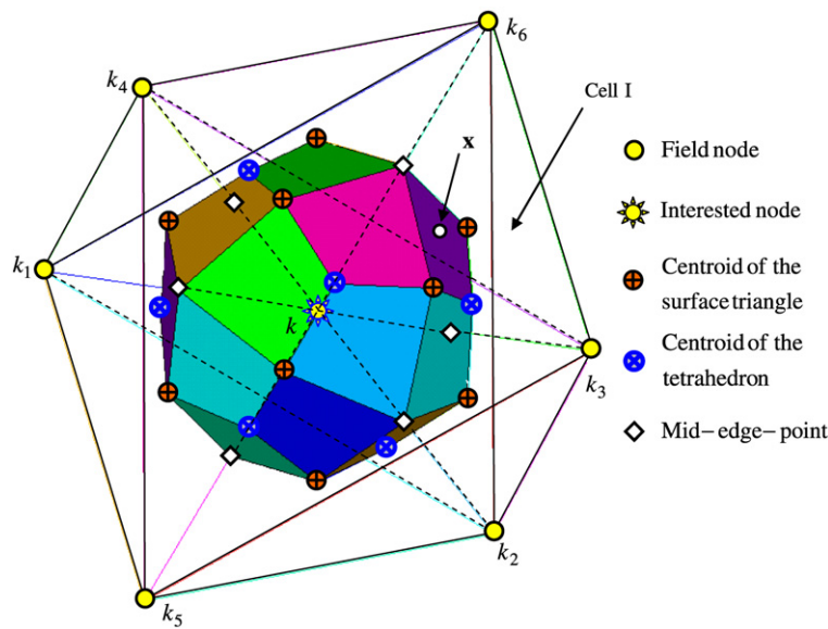
Fig. 1. A typical node-based 3D smoothing domain for node k .
