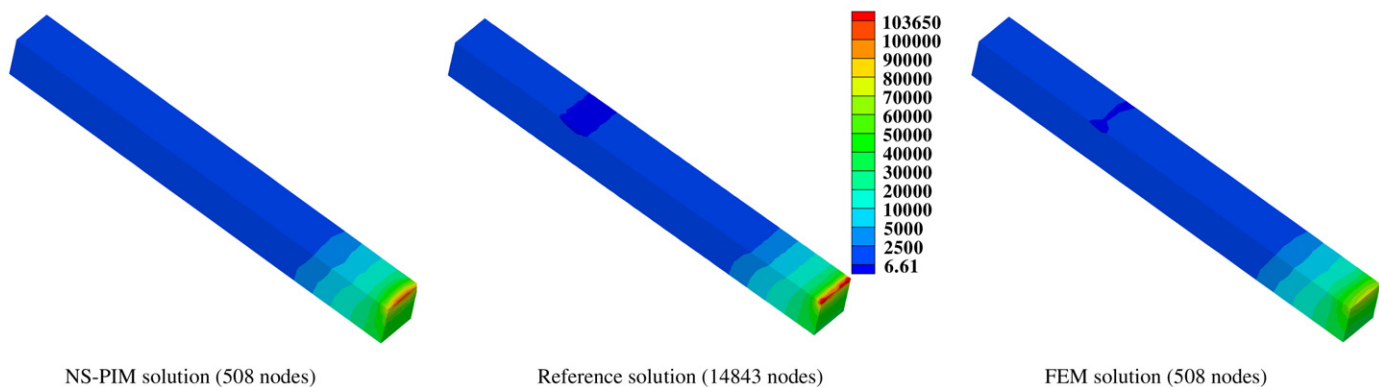
Fig. 5. Comparison of the z component of temperature gradients.
