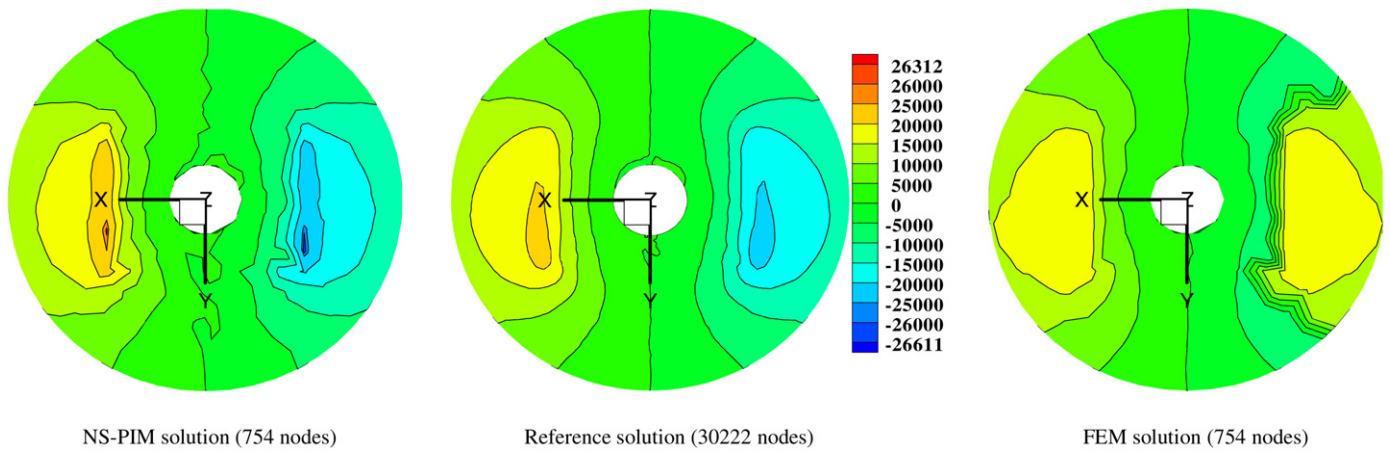
Fig. 9. Comparison of temperature gradients in y-direction.
