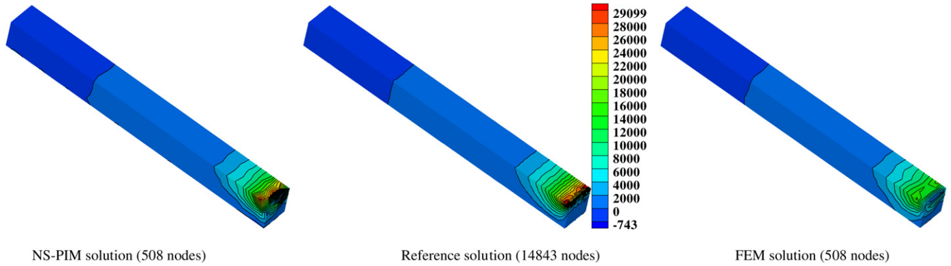
Fig. 4. Comparison of the y component of temperature gradients.
