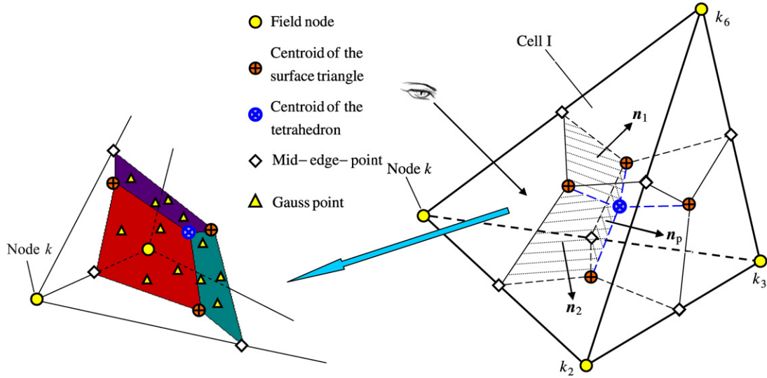
Fig. 2. The schematic of one portion of a node-based smoothing domain for node k located in a four-node tetrahedral cell I ( k-k_2-k_3-k_6 ).
